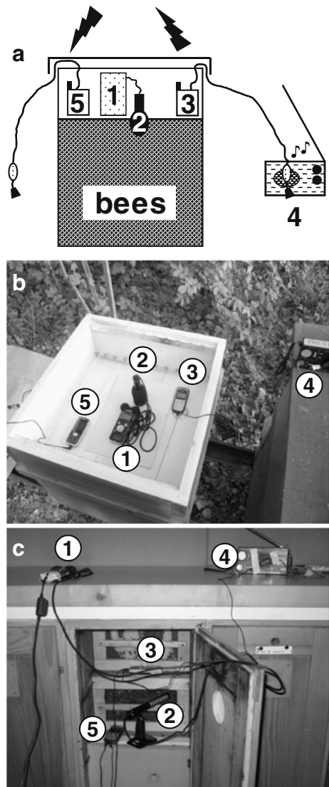
Figure 1. Apparatus positioning in the different hives. a Schematic drawing. Sound recorder 1 was connected to a microphone 2, the latter was placed in the close vicinity of the bees in the hive. The first (emitting) mobile phone 3 was connected with hands-free kit, the latter having its small microphone maintained on the loudspeaker of a radio apparatus 4. A second (receiving) mobile phone 5, also having a hands-free kit, was also kept inside the hive. The use of the radio apparatus is intended to allow a permanent communication between the two mobile phone handsets, in order to avoid unwanted disconnection after a while. b Image of a Dadant-Blatt model of beehive. The microphone is placed through the upper nourishing hole. c Image of a Swiss Bürki model of beehive. The microphone was placed behind a board having a grid instead of a glass plate. During the experiments, the door of the Bürki hive was closed and the Dadant-Blatt hive was covered with the roof. A similar positioning can be easily performed with other types of beehives.
